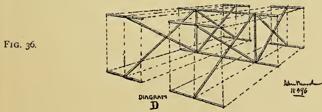
FIGS. 33-37.—The Funny Hargrave Kite.
